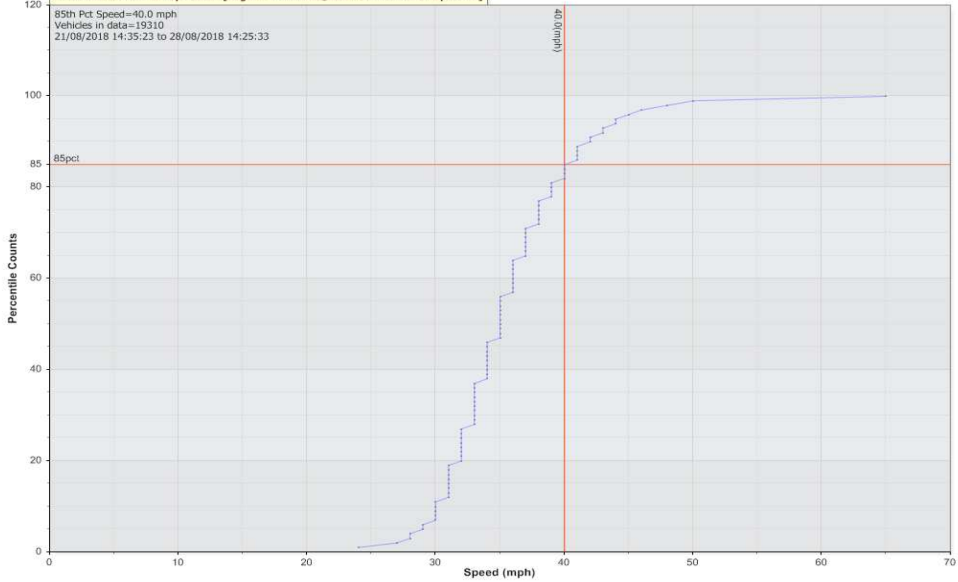
Percentile Counts Vs. Speed for [LogHIL-PottonRd@VAS: Outbound to Papworth]
