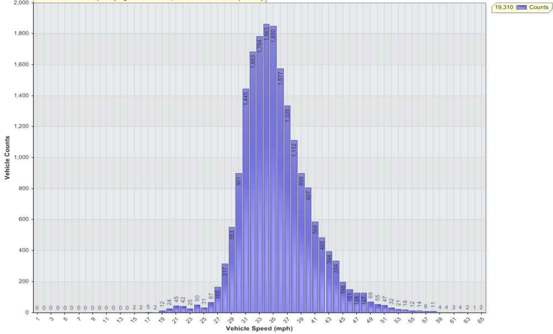
Vehicle Counts Vs. Speed [LogHIL-PottonRd@VAS: Outbound to Papworth]
